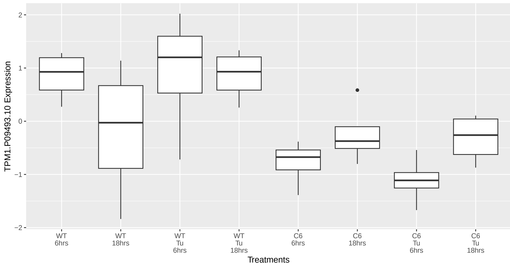
TPM1.P09493.10 occurs in the magenta module
