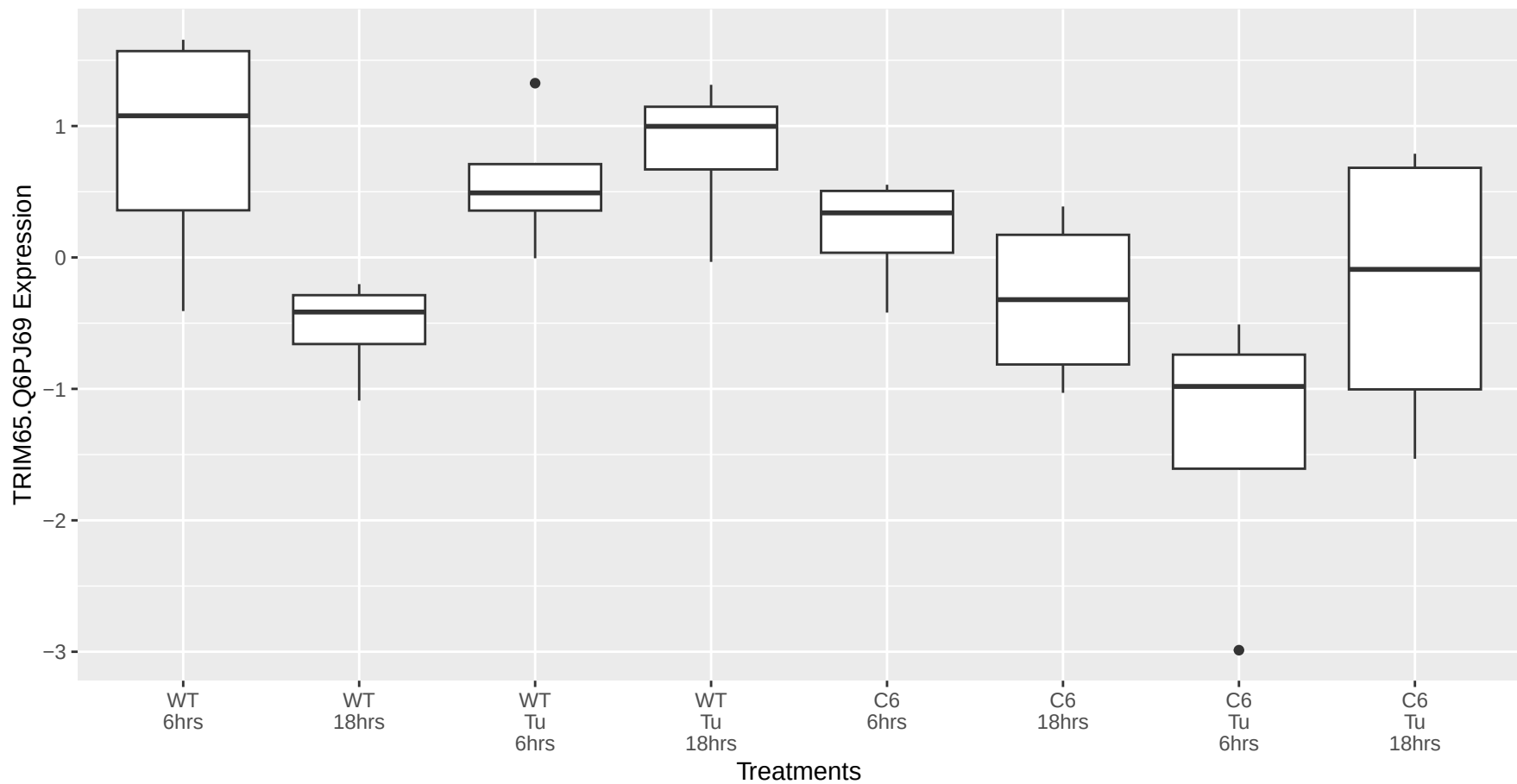
TRIM65.Q6PJ69 occurs in the magenta module
