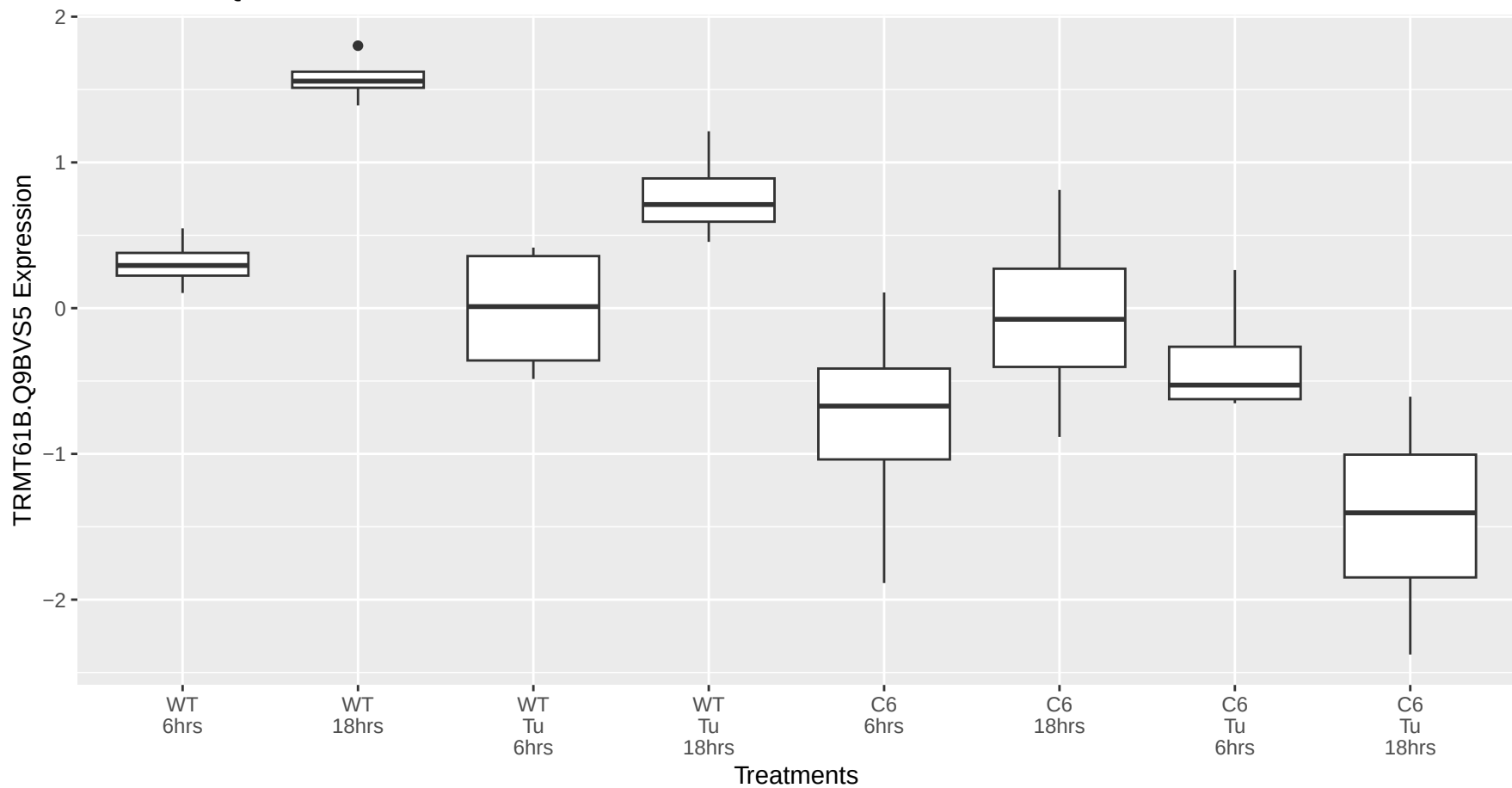
TRMT61B.Q9BVS5 occurs in the brown module
