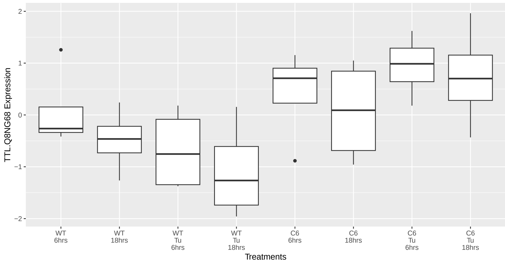
TTL.Q8NG68 occurs in the red module
