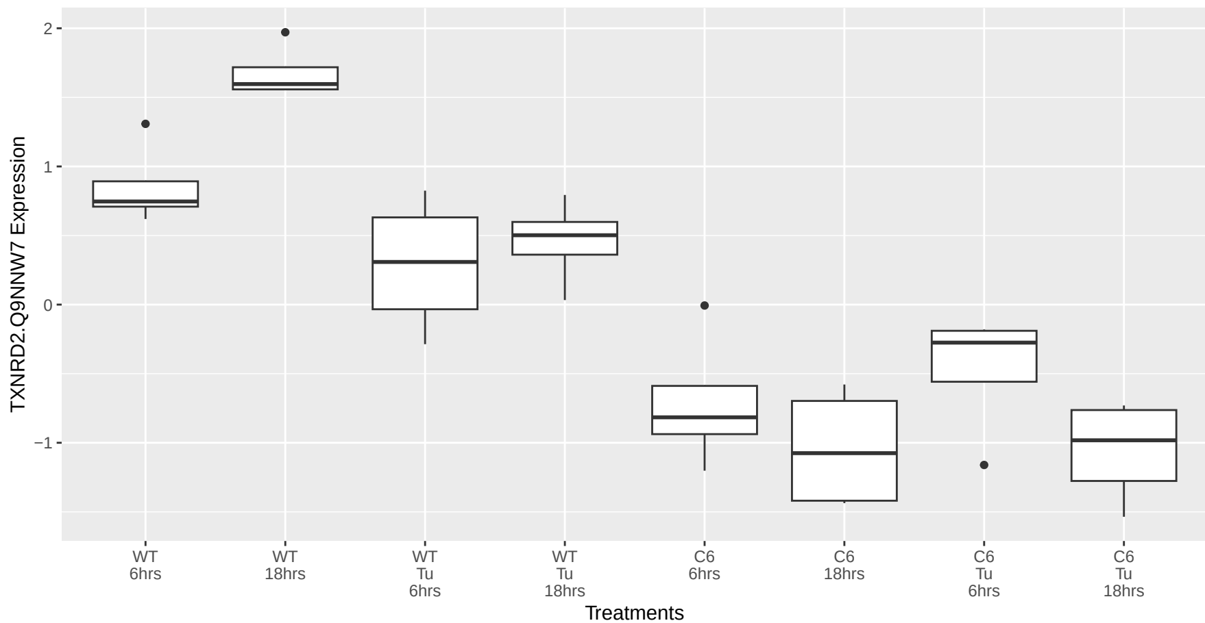
TXNRD2.Q9NNW7 occurs in the brown module
