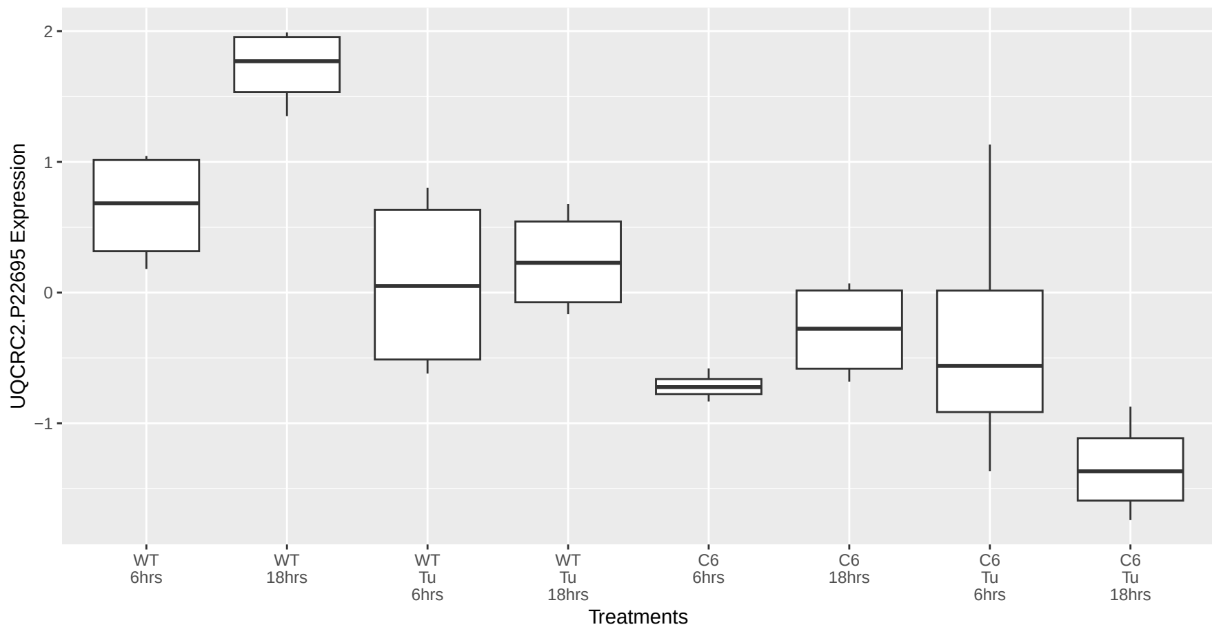
UQCRC2.P22695 occurs in the brown module
