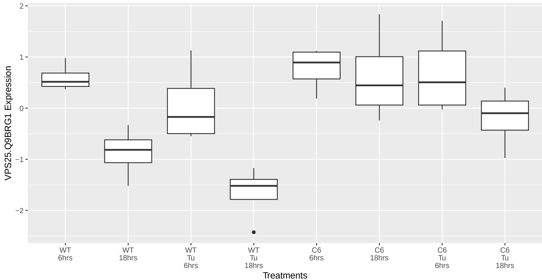
VPS25.Q9BRG1 occurs in the cyan module
