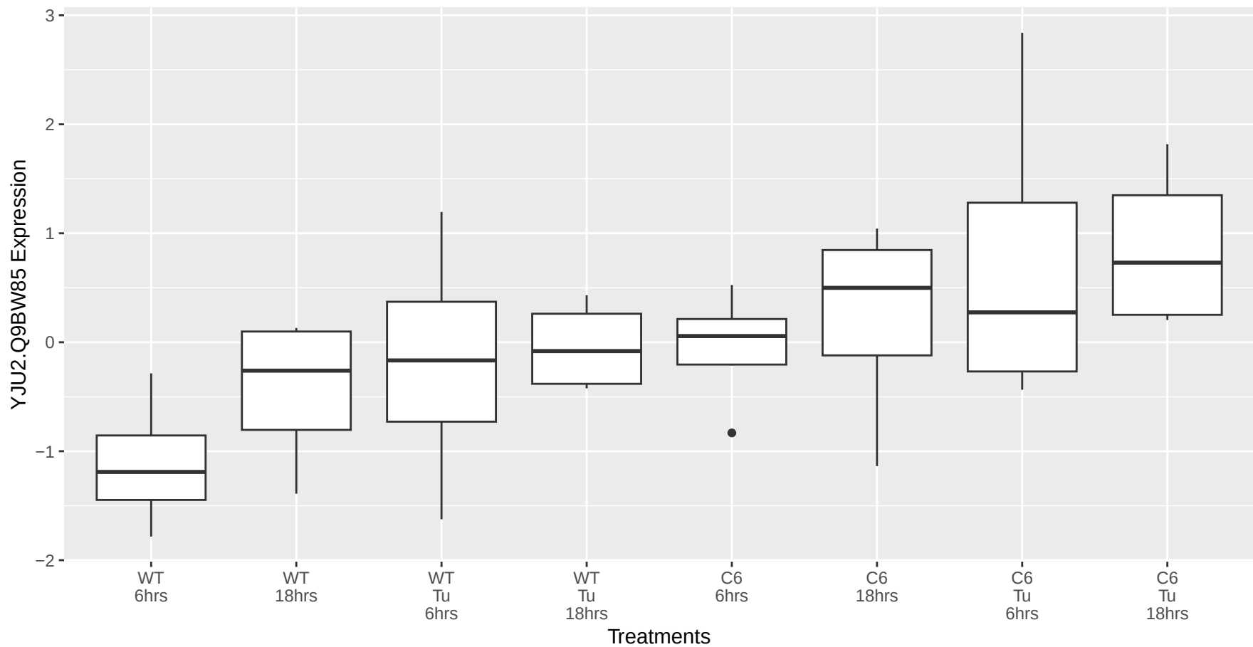
YJU2.Q9BW85 occurs in the magenta module
