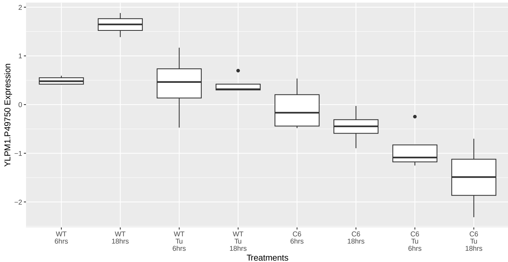
YLPM1.P49750 occurs in the magenta module
