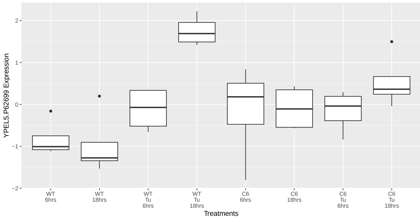
YPEL5.P62699 occurs in the pink module
