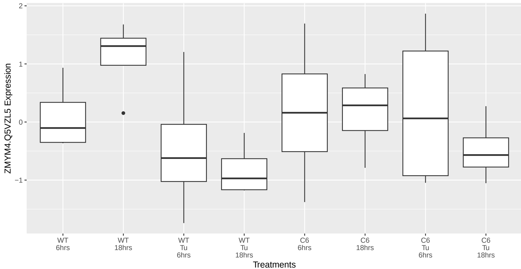
ZMYM4.Q5VZL5 occurs in the black module
