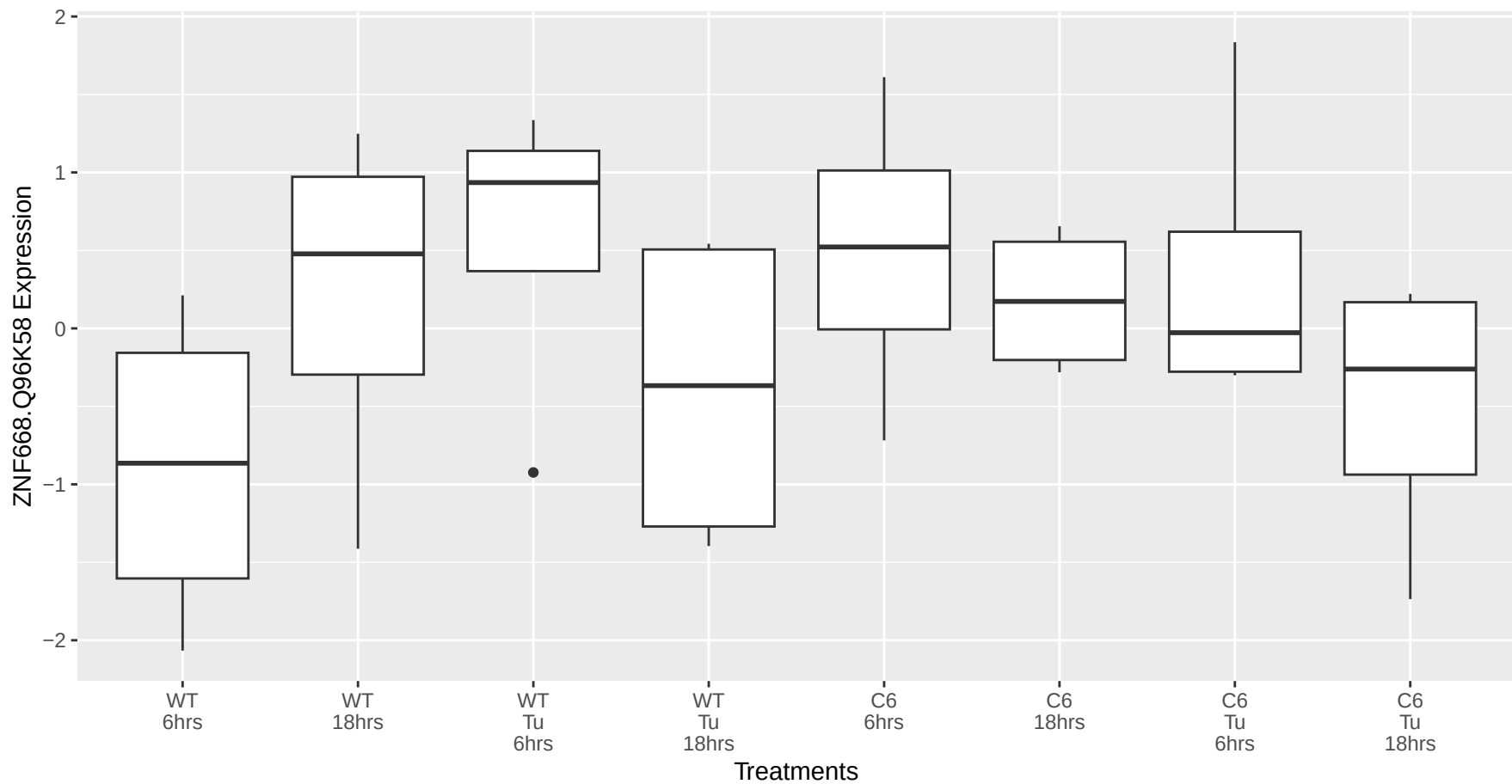
ZNF668.Q96K58 occurs in the black module
