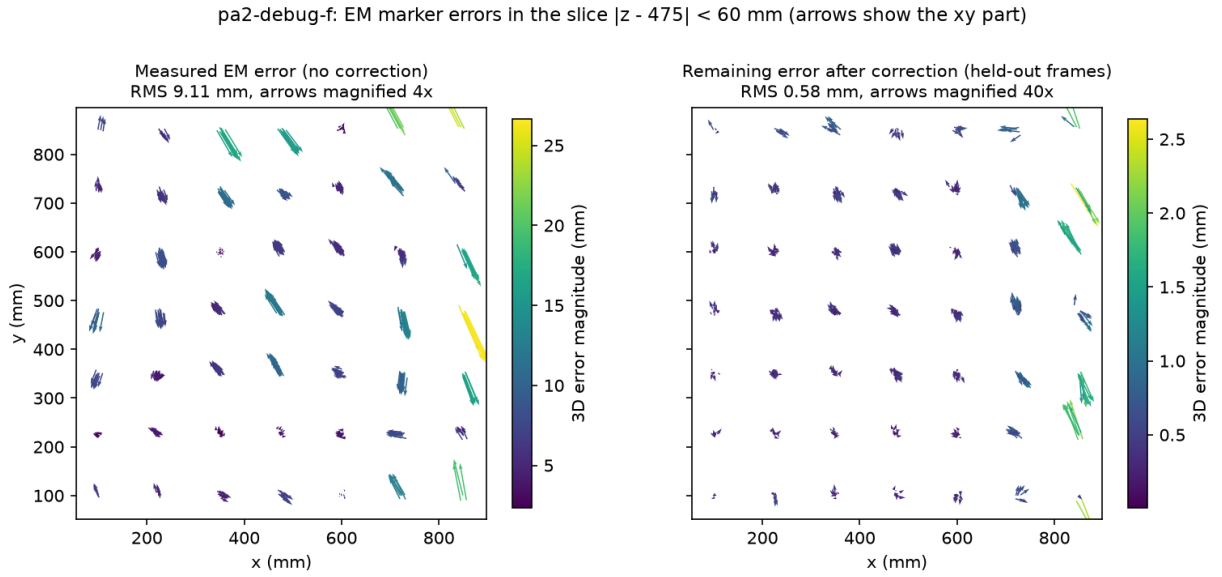
Figure 6: Distortion in a slice of pa2-debug-f before and after correction (held-out frames).
