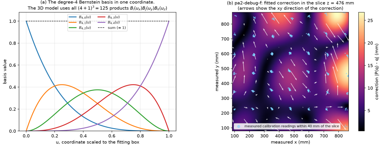
Figure 3: The degree-4 Bernstein basis, and the magnitude of the fitted correction |P(\vec{q}) - \vec{q}| in a horizontal slice of pa2-debug-f with the nearby calibration readings.
