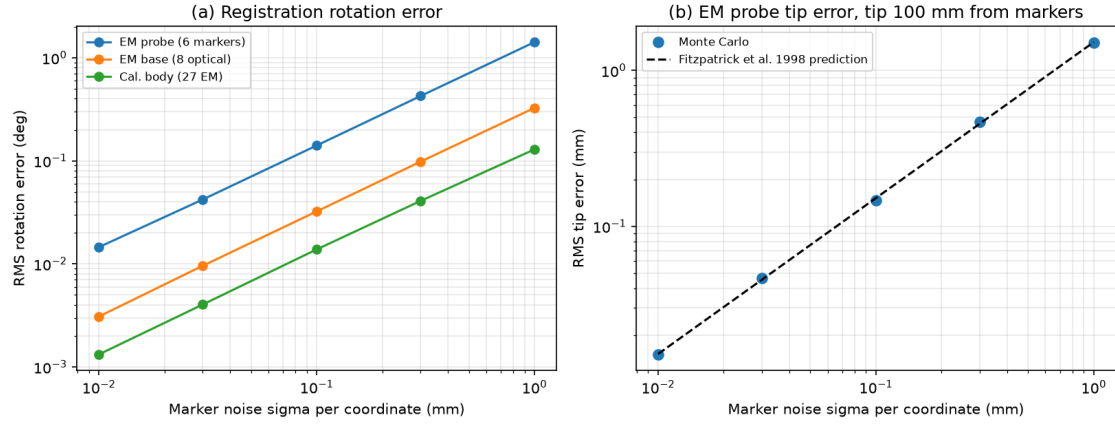
Figure 7: Registration error against marker noise; tip error compared with the Fitzpatrick prediction.
