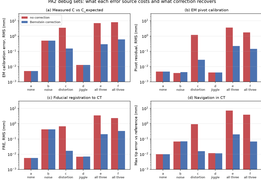
Figure 4: PA2 debug sets with and without distortion correction (log scale).
