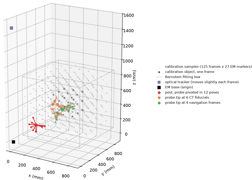
Figure 1: The PA2 scene for pa2-debug-f in EM tracker coordinates: calibration samples and fitting box, the optical tracker, the probe pivoting on the post, and the probe at the CT fiducials and navigation targets.
