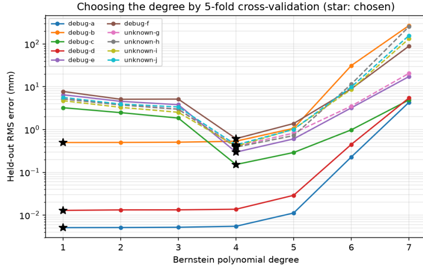
Figure 5: Held-out correction error against Bernstein degree for all PA2 sets.
