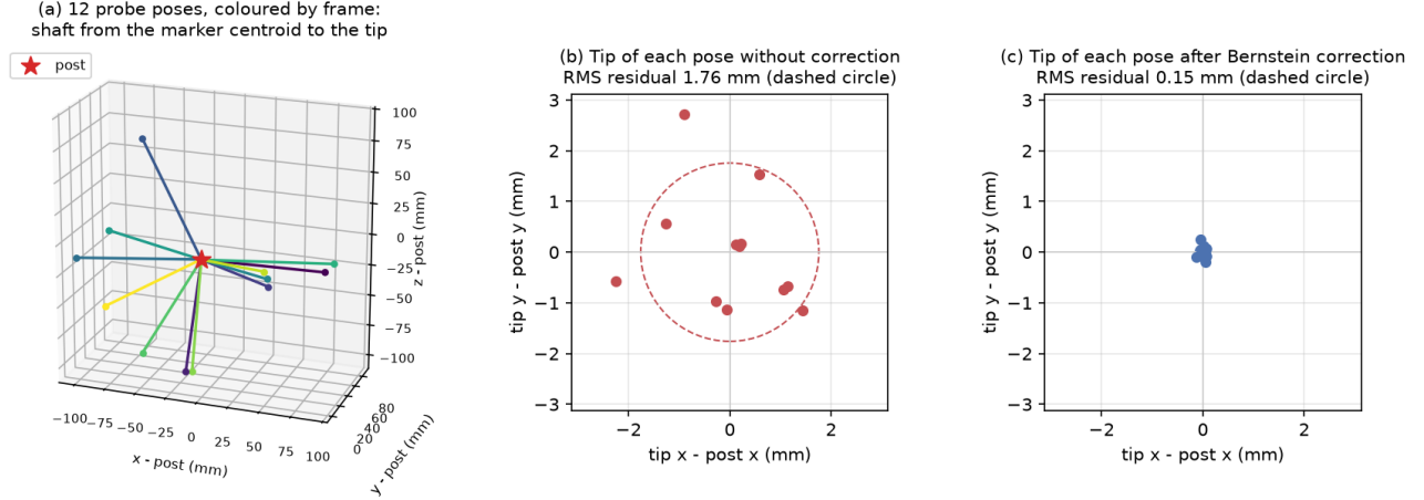
Figure 2: EM pivot calibration of pa2-debug-f: the 12 probe poses around the post, and each pose’s tip relative to the post without and with distortion correction.
