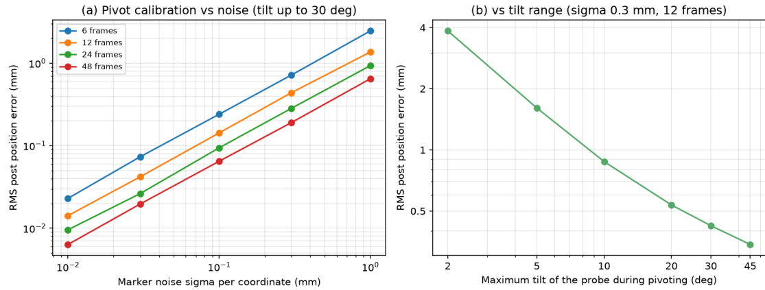
Figure 8: Pivot calibration post error against noise, number of frames and tilt range.
