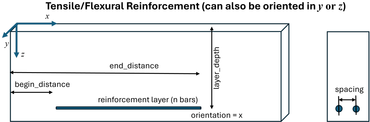
Figure 10: Parametrization of longitudinal flexural and tensile reinforcement layers.
