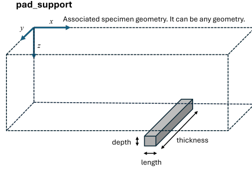
Figure 16: Parametrization of deformable pad supports.
