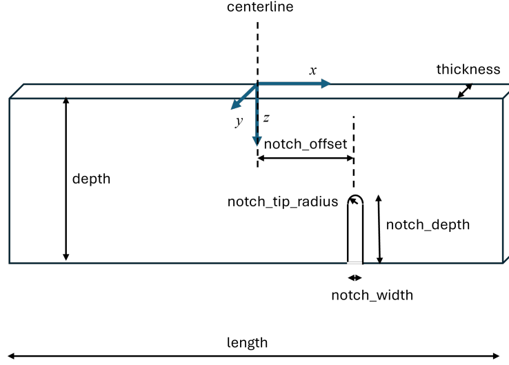
Figure 6: Notched prism parametrization
