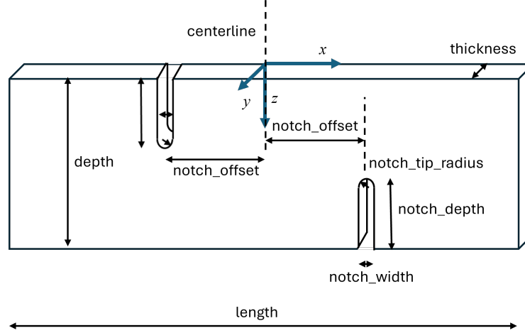
Figure 4: Doubly notched prism parametrization
