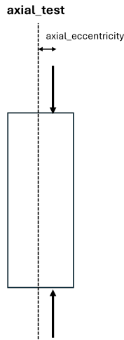
Figure 15: Parametrization of the axial loading test with eccentricity.
