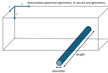
Figure 17: Parametrization of cylindrical roller supports.
