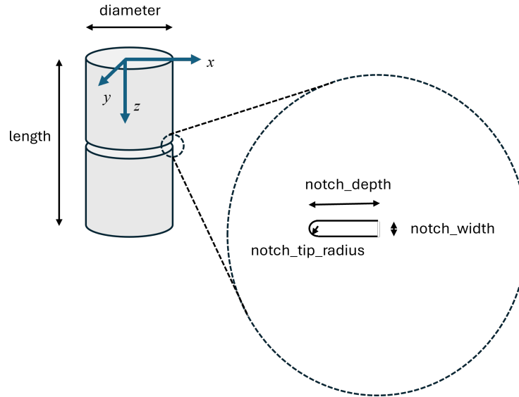
Figure 8: Notched cylinder parametrization
