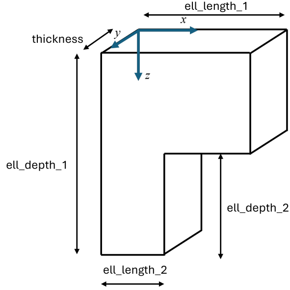
Figure 7: Ell shape parametrization
