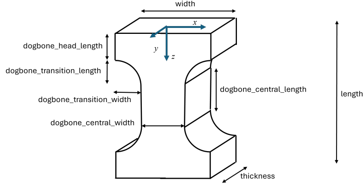
Figure 5: Dogbone parametrization
