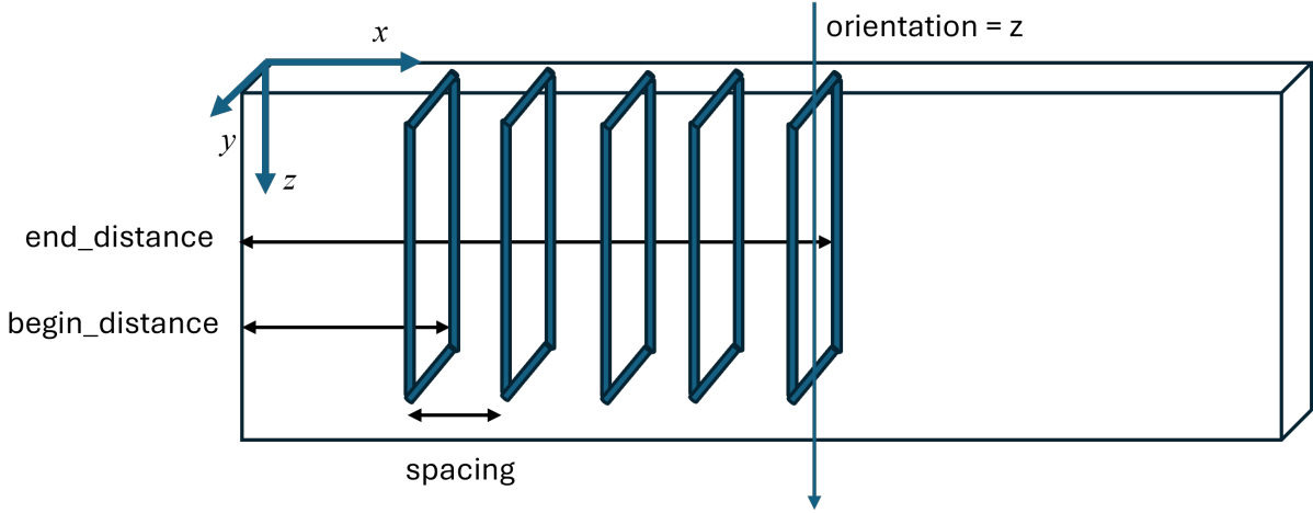
Figure 11: Parametrization of stirrups and ties reinforcement systems.
