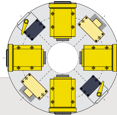
Loading D 745 – 8-fold pitch
