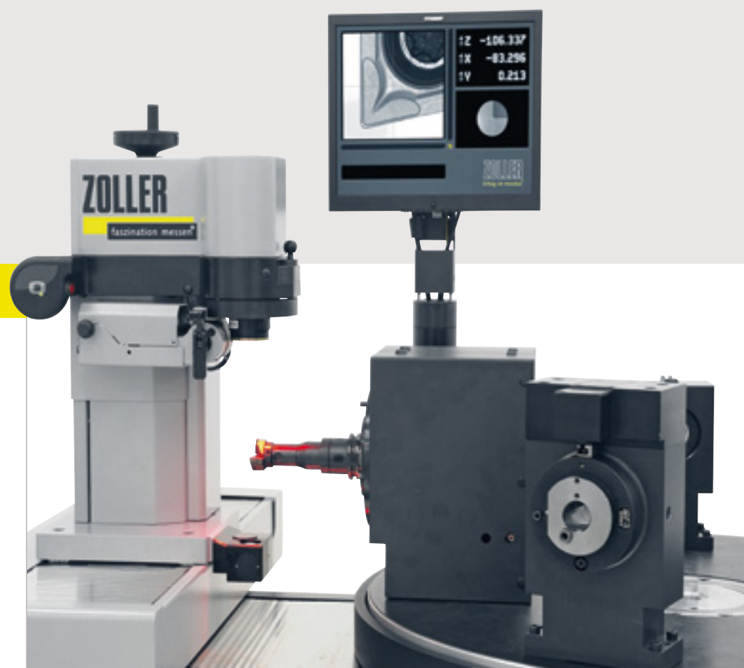
Optic adjustment \pm 50 mm, manual adjustment via hand wheel
