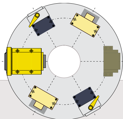
Loading D 745 – 6-fold pitch
