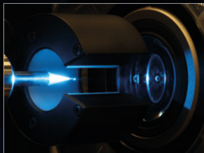
»pomLightTube« and coaxial lighting for high-precision measurement
