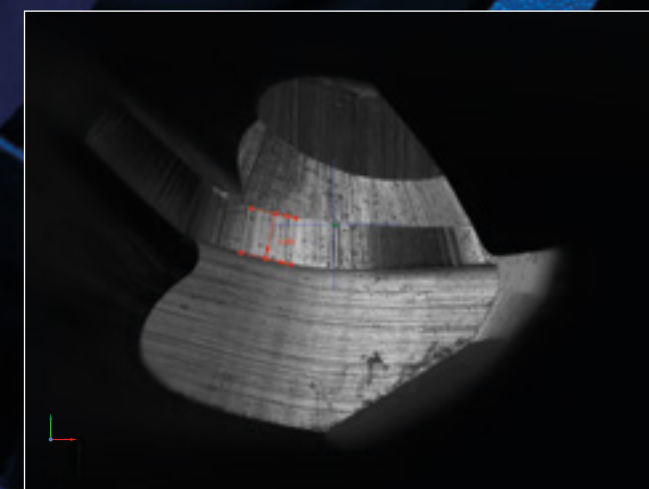
Inspection of a full radius cutter D 0.6 mm
