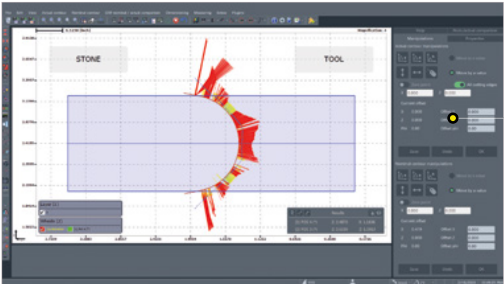
Intelligent »lasso« function – enables tool areas to be marked intuitively and precisely to be captured.
