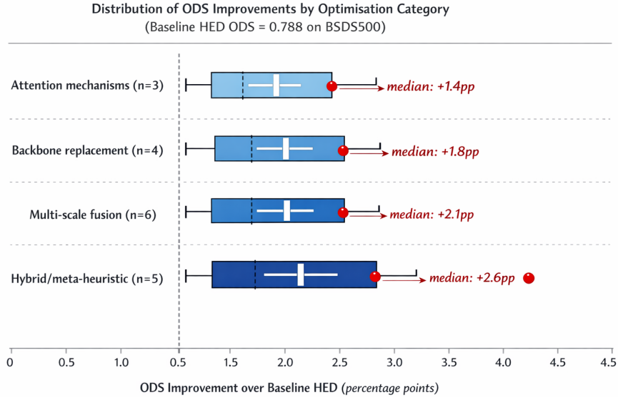
Figure 4: Distribution of ODS improvements over baseline HED (0.788) by optimisation category. Box plots show median, IQR, and outliers; numbers indicate study count per category.
