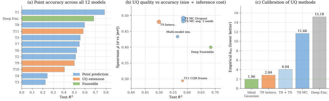
Figure 5.5.: Master summary of the twelve GNN-based and uncertainty-aware models evaluated in this thesis. Panel (a) sorts trials by test R^2 (point-prediction trials blue, uncertainty-aware extensions orange, Deep Ensemble green); the Deep Ensemble leads UQ-compatible models at R^2 = 0.6841 . Panel (b) is the accuracy/UQ trade-off ( R^2 vs Spearman \rho , marker size proportional to log inference cost): Deep Ensemble and MC Dropout sit on opposite corners; T11 (frozen-backbone CQR) occupies an attractive low-cost corner. Panel (c) compares k_{95} (lower is better, Gaussian ideal 1.96); T9 is closest to ideal among trained models.
