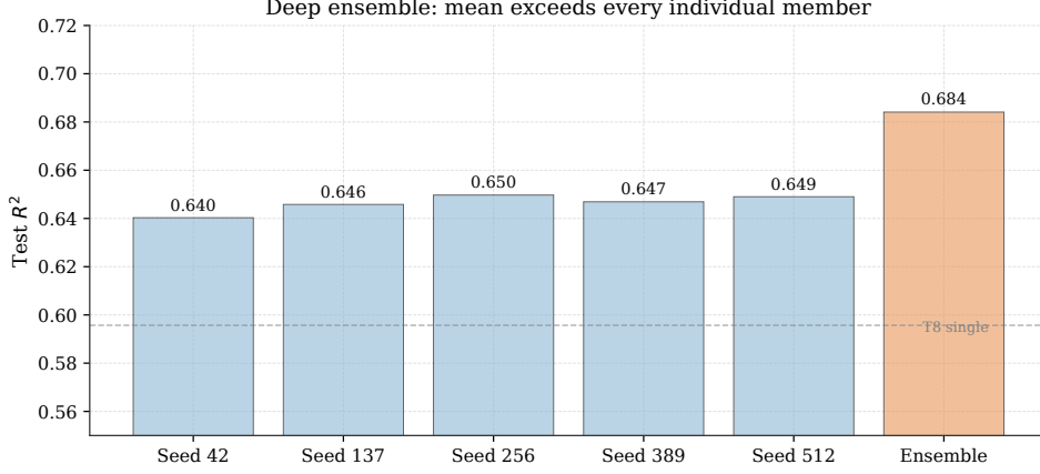
Figure 5.4.: Deep Ensemble: mean exceeds every individual member.
