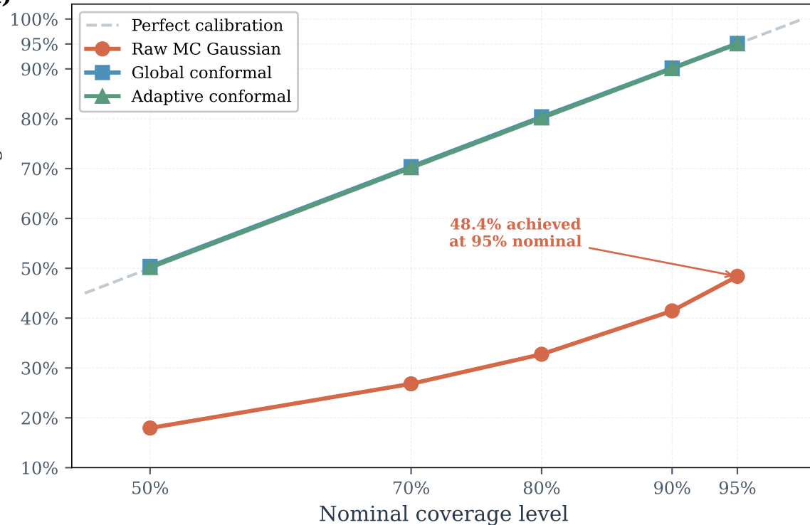
Calibration Curve
