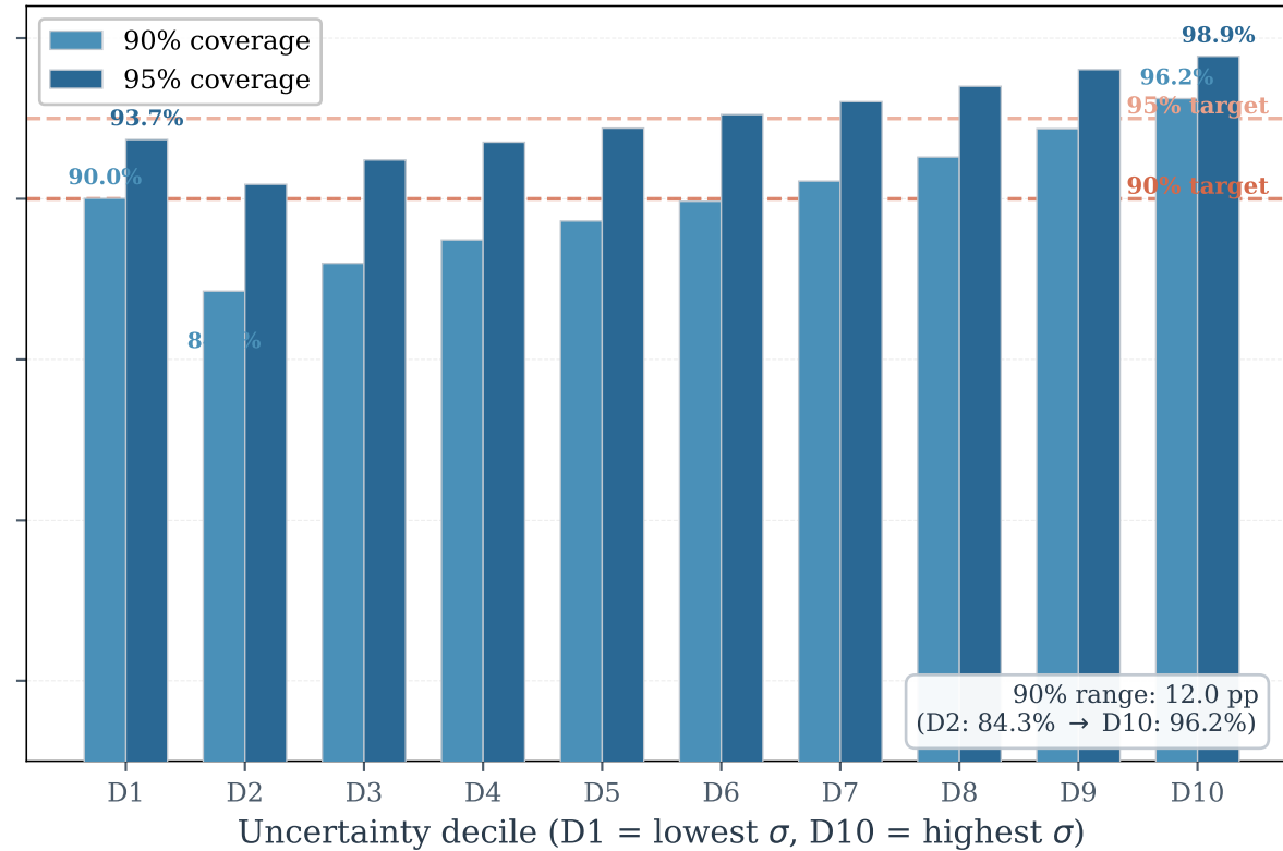
Adaptive Conformal ( \sigma -normalized)
