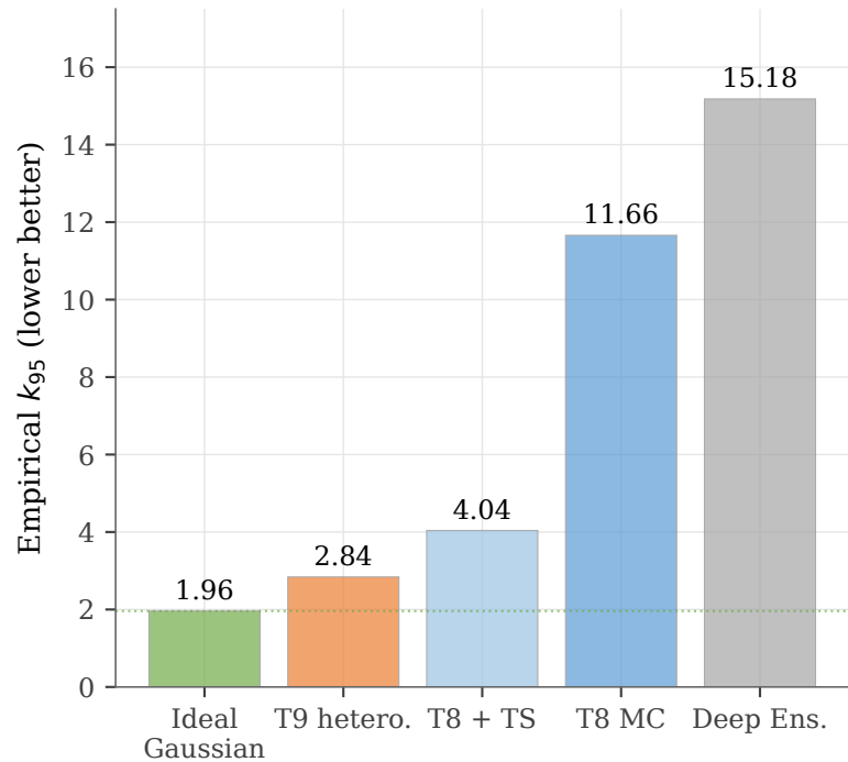
(c) Calibration of UQ methods
