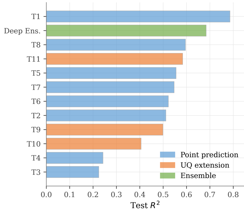
(a) Point accuracy across all 12 models
