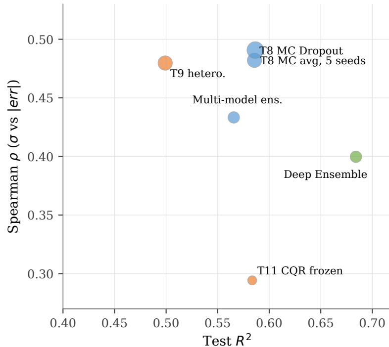
(b) UQ quality vs accuracy (size \propto inference cost)
