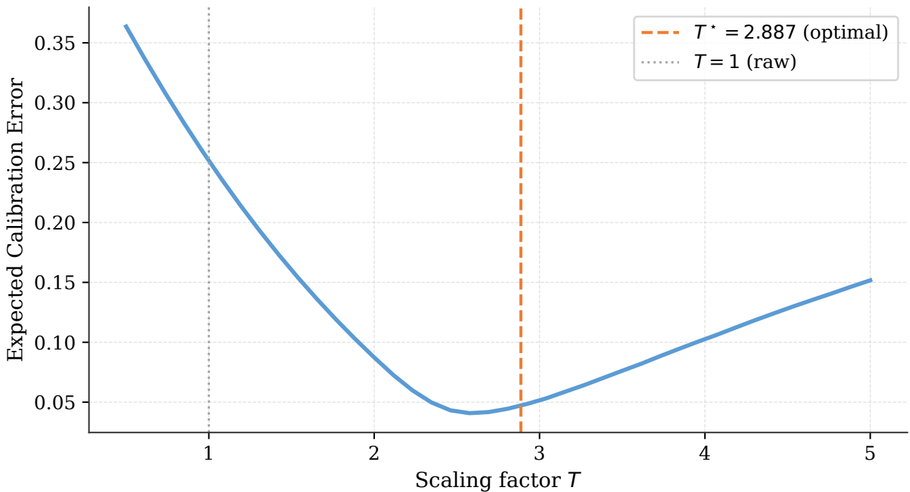
ECE optimisation for T8 MC Dropout regression \sigma -scaling
