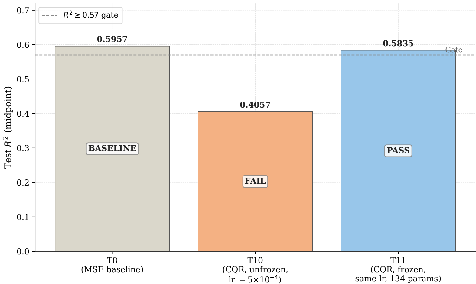
CQR R^2 progression: only frozen-backbone training (T11) preserves accuracy
