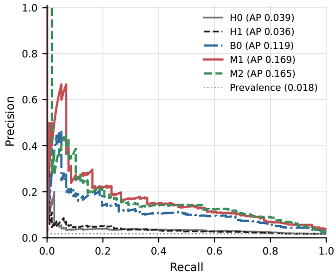
B Precision-recall
