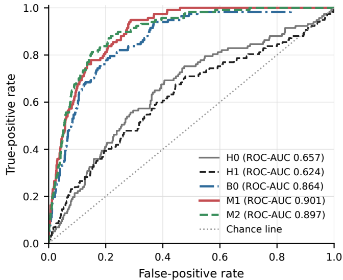
A ROC
