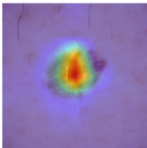
Grad-CAM M2=0.005
