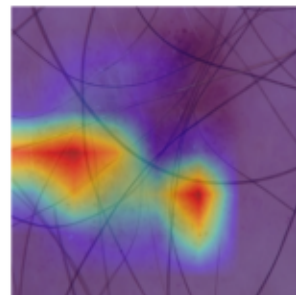
Grad-CAM M2=0.063
