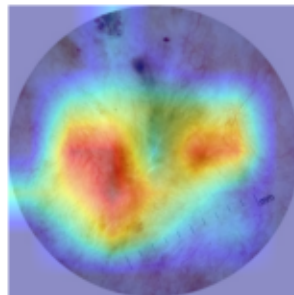
Grad-CAM M2=0.979
