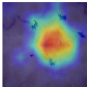
Grad-CAM M2=0.977
