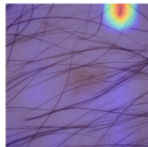
Grad-CAM M2=0.002
