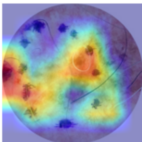
Grad-CAM M2=0.978
