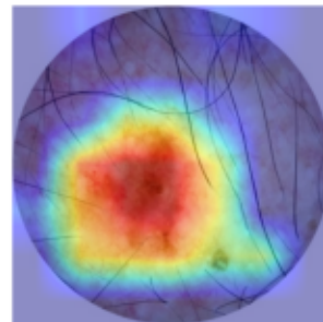
Grad-CAM M2=0.971
