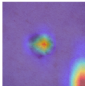
Grad-CAM M2=0.009
