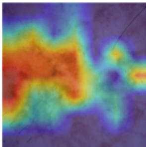
Grad-CAM M2=0.980
