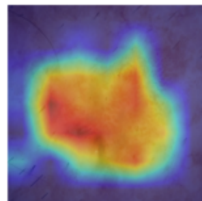
Grad-CAM M2=0.976
