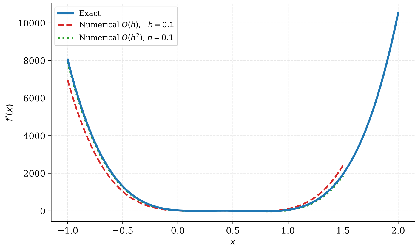
Numerical vs Exact — 1st Derivative ( h = 0.1 )
