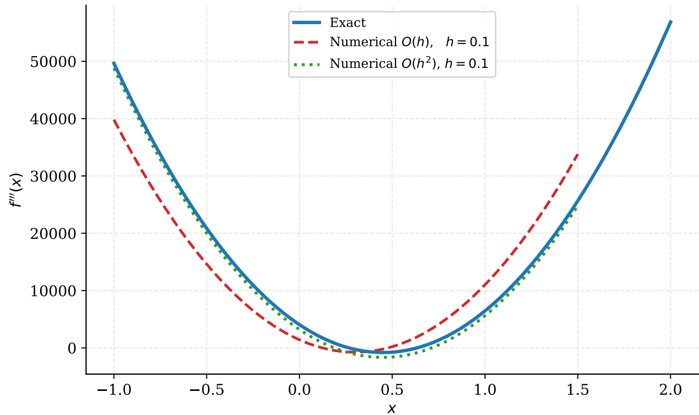
Numerical vs Exact — 3rd Derivative ( h = 0.1 )
