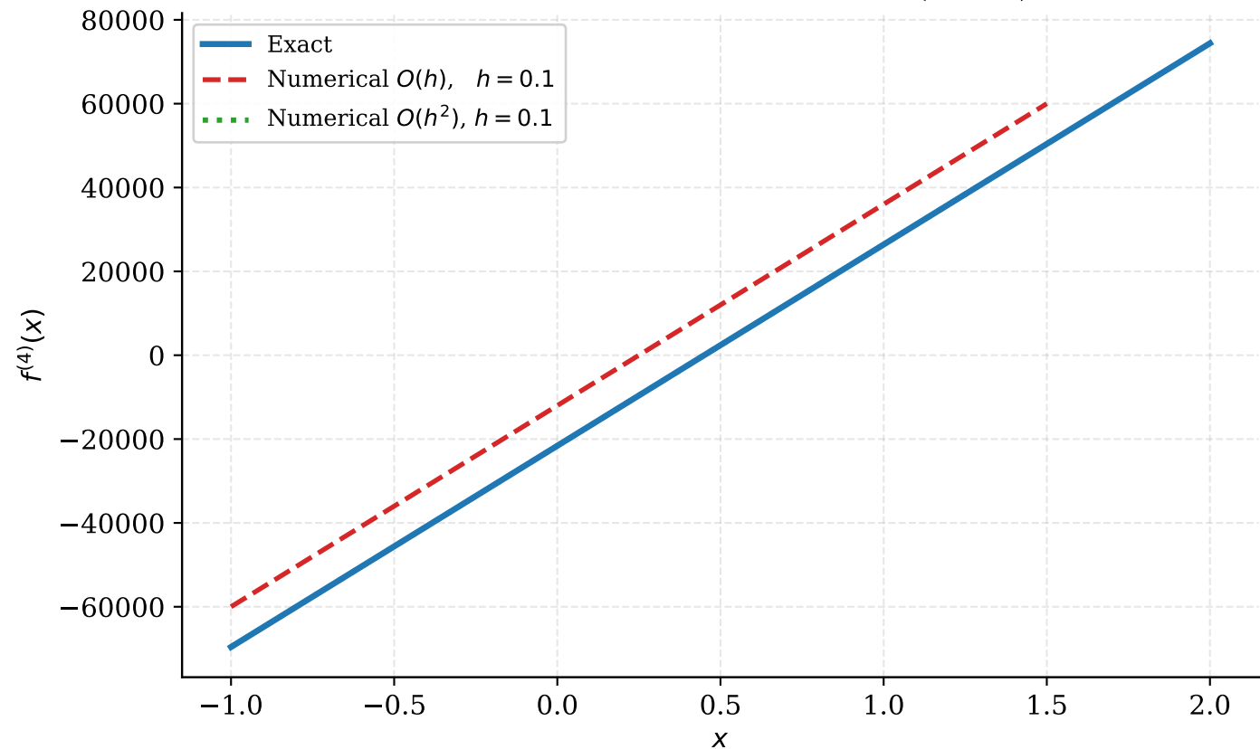
Numerical vs Exact — 4th Derivative ( h = 0.1 )
