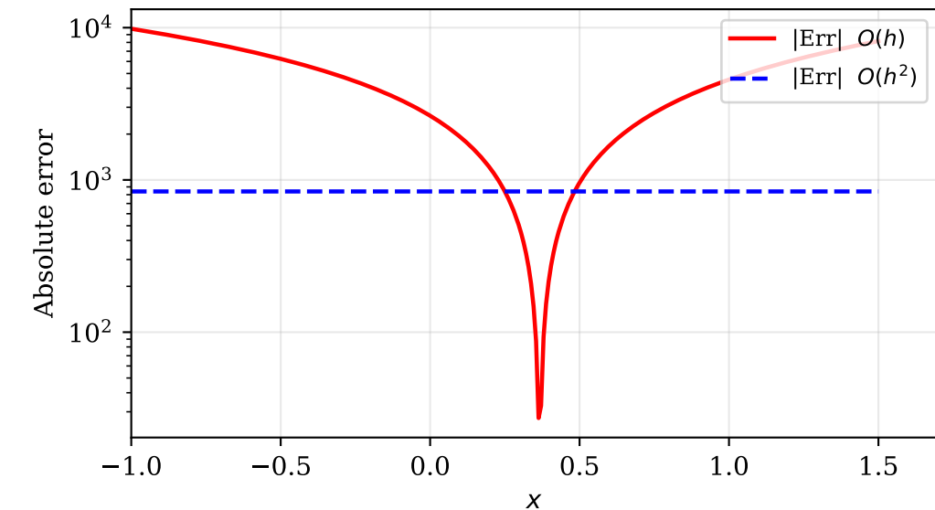
3rd Derivative — Absolute Error ( h = 0.1 )
