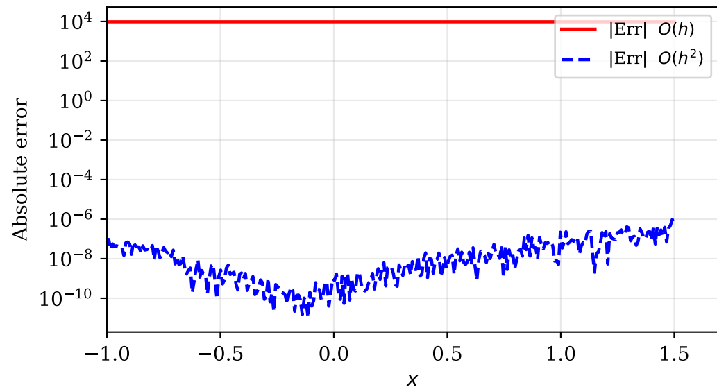
4th Derivative — Absolute Error ( h = 0.1 )
