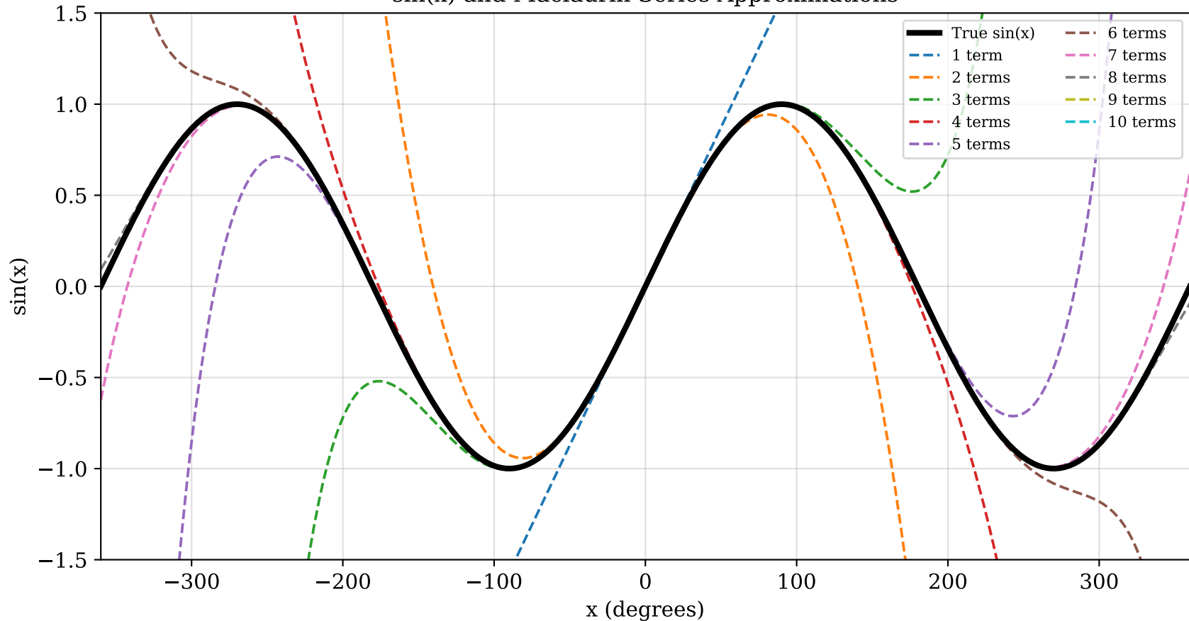
\sin(x) and Maclaurin Series Approximations
