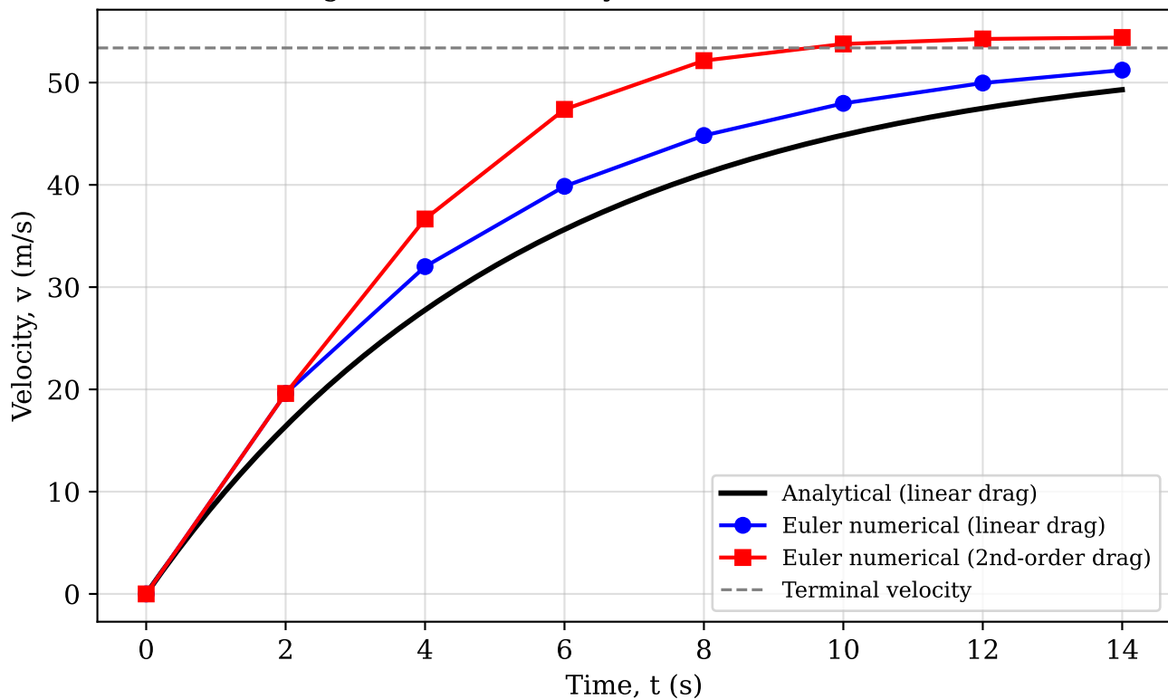
Falling Parachutist: Analytical vs. Numerical Solution
