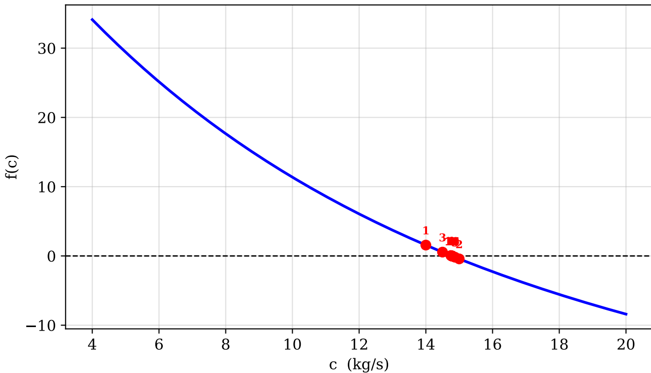
Bisection - Parachutist Drag Coefficient (Iteration markers labelled)
