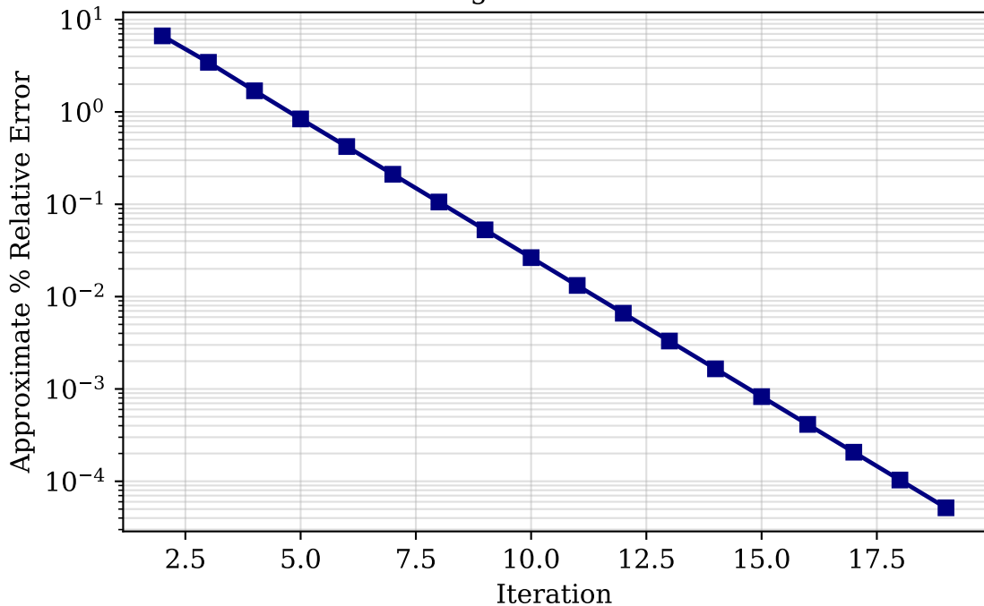
Bisection Convergence - Parachutist Problem
