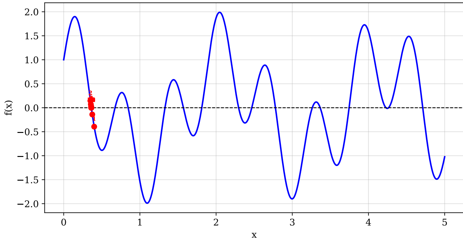
Bisection on f(x) = \sin(10x) + \cos(3x) [bracket 0.3-0.5]
