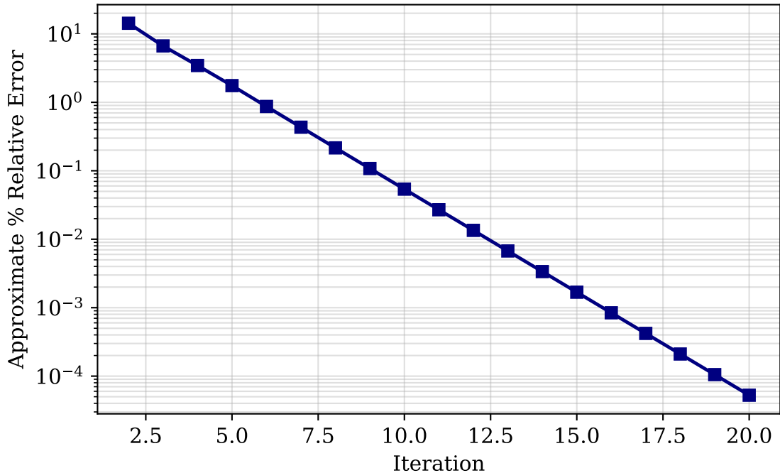
Bisection Convergence - f(x) = \sin(10x) + \cos(3x)
