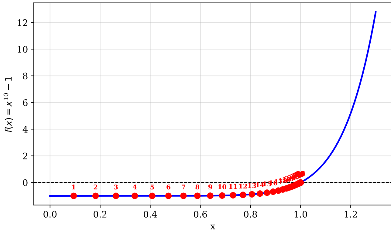
False Position - f(x) = x^{10} - 1 (Stagnation Demo)
