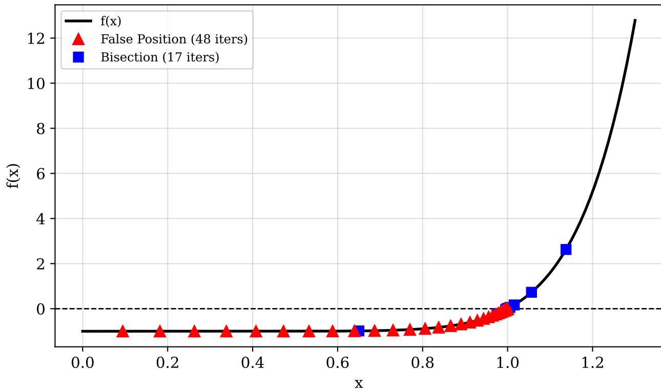
Root Approximations: FP vs Bisection on x^{10} - 1
