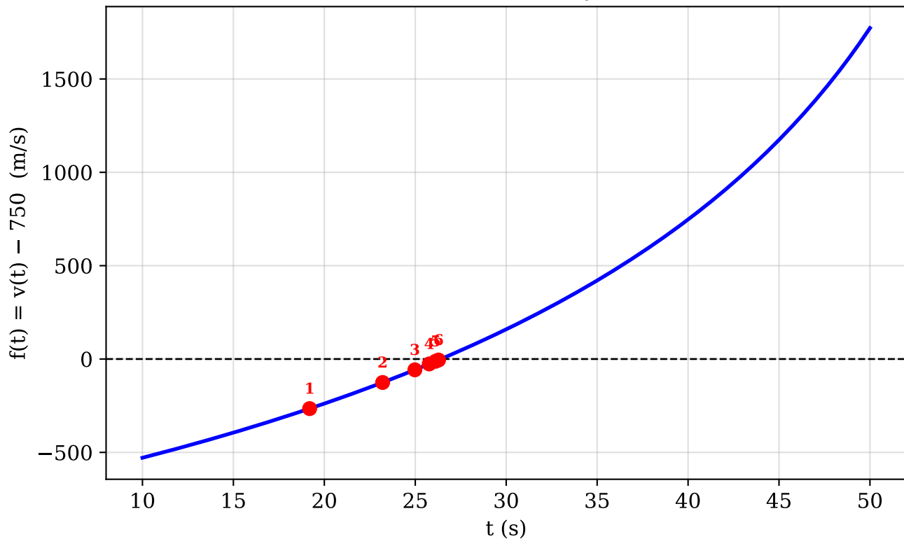
False Position - Rocket Velocity (Problem 5.20)
