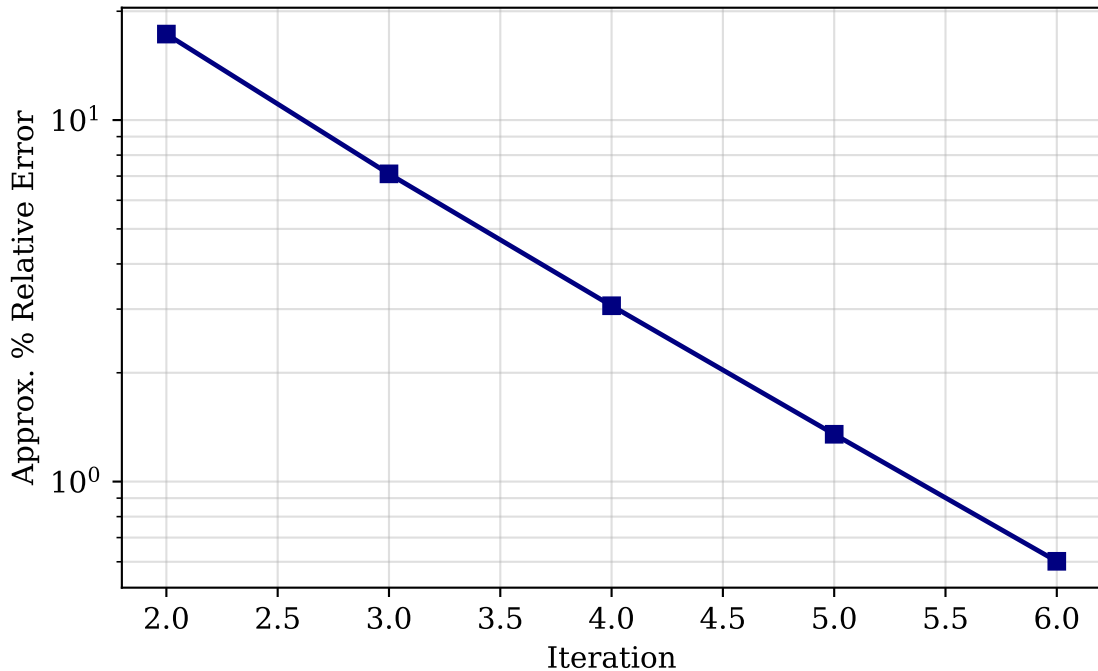
False Position Convergence - Rocket Problem
