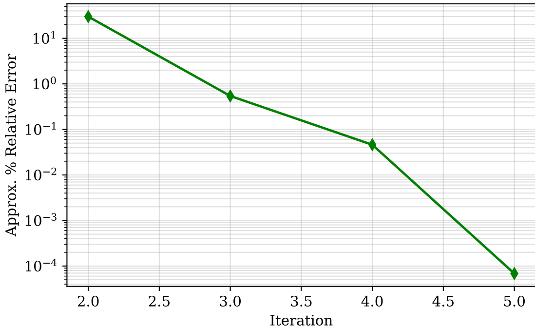
False Position Convergence - Floating Sphere
