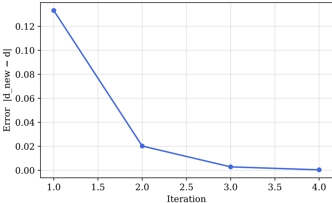
Fixed-Point Iteration - Convergence (Spring-Mass)
