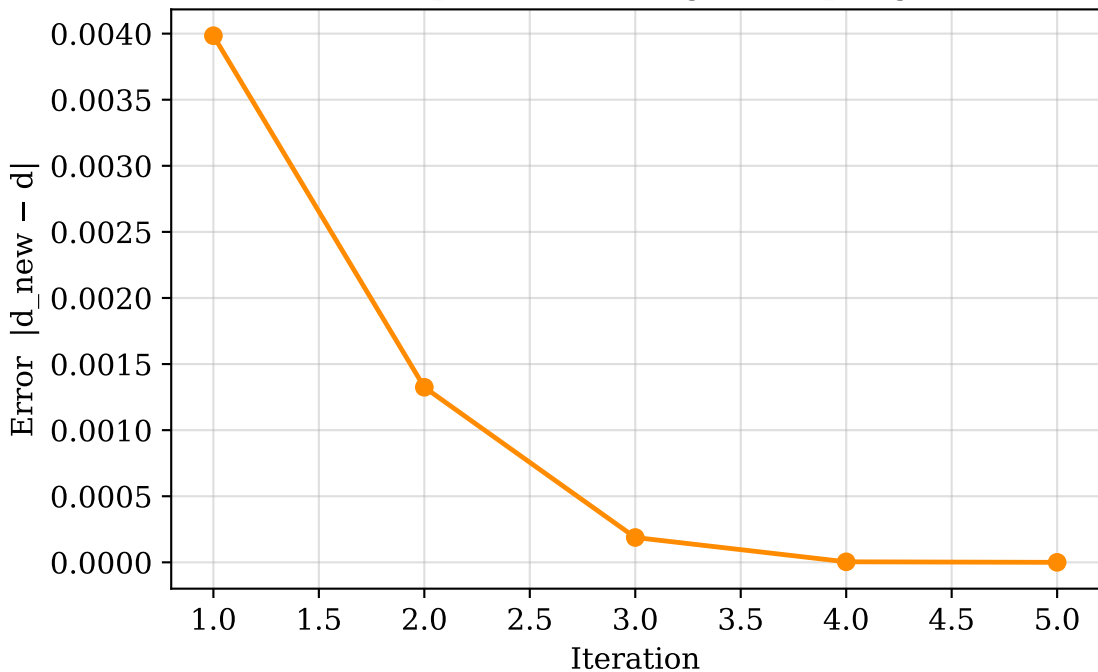
Newton-Raphson - Convergence (Spring-Mass)
