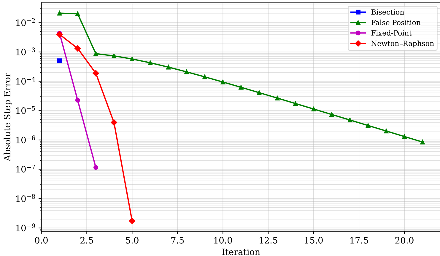
Convergence Comparison - All Four Methods (Spring-Mass Problem)
