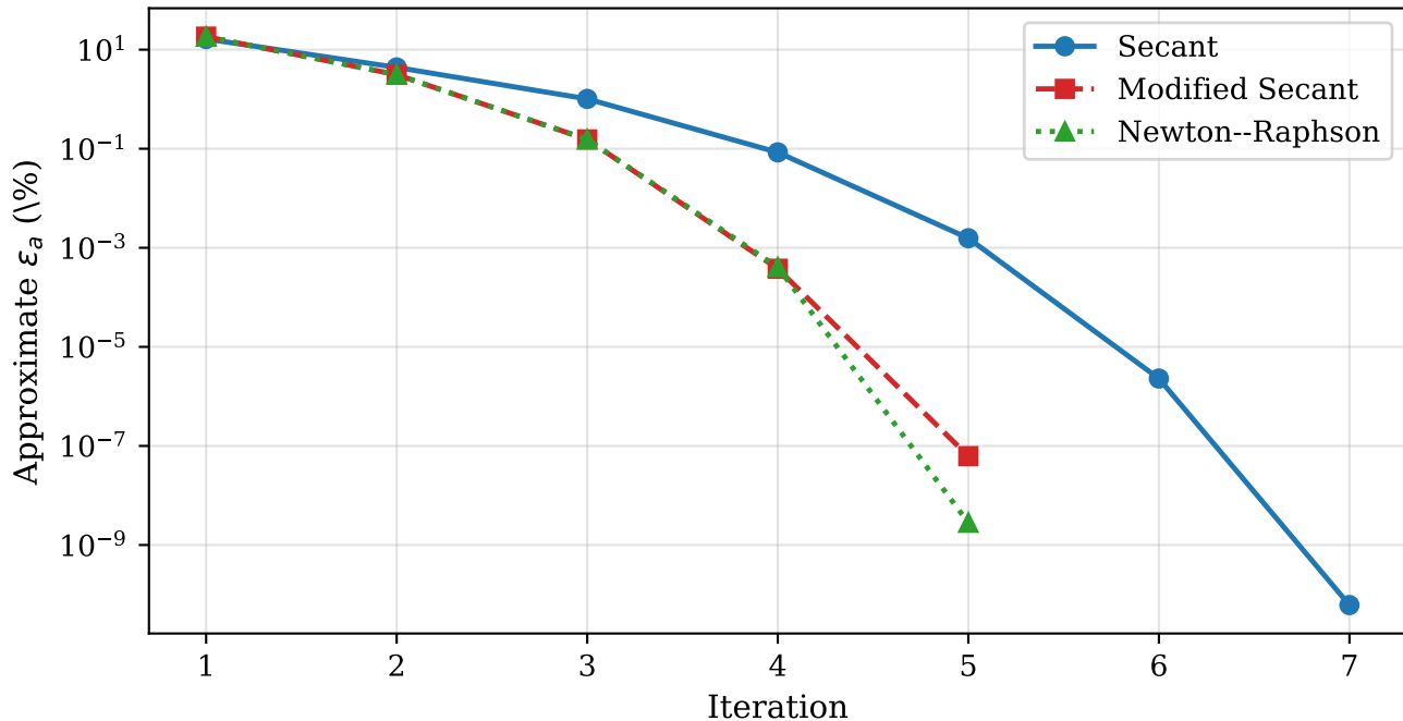
Error Convergence — Root 1 ( \theta^* \approx 37.96^\circ )
