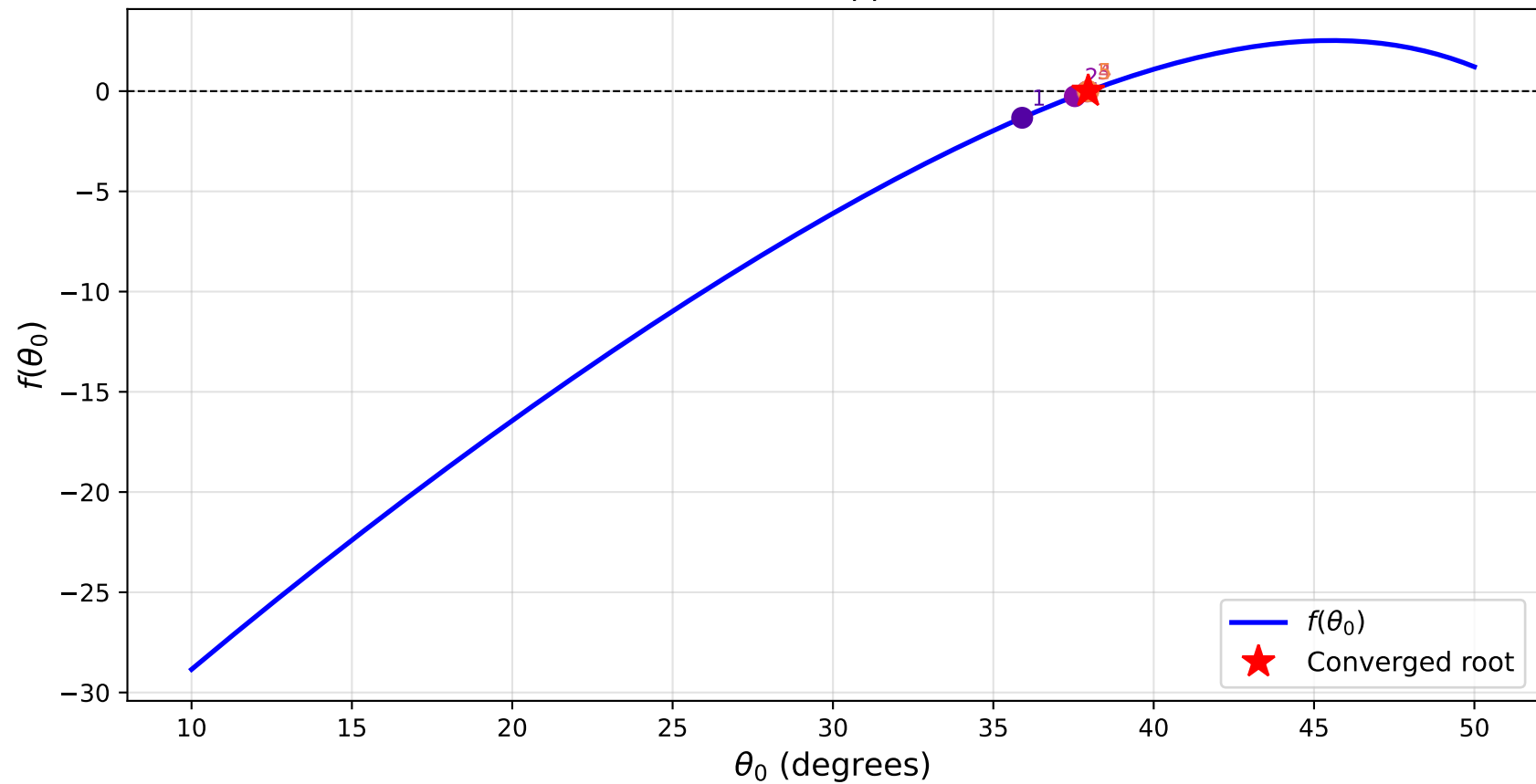
Secant Method: Root 1 Approximations on f(\theta_0)
