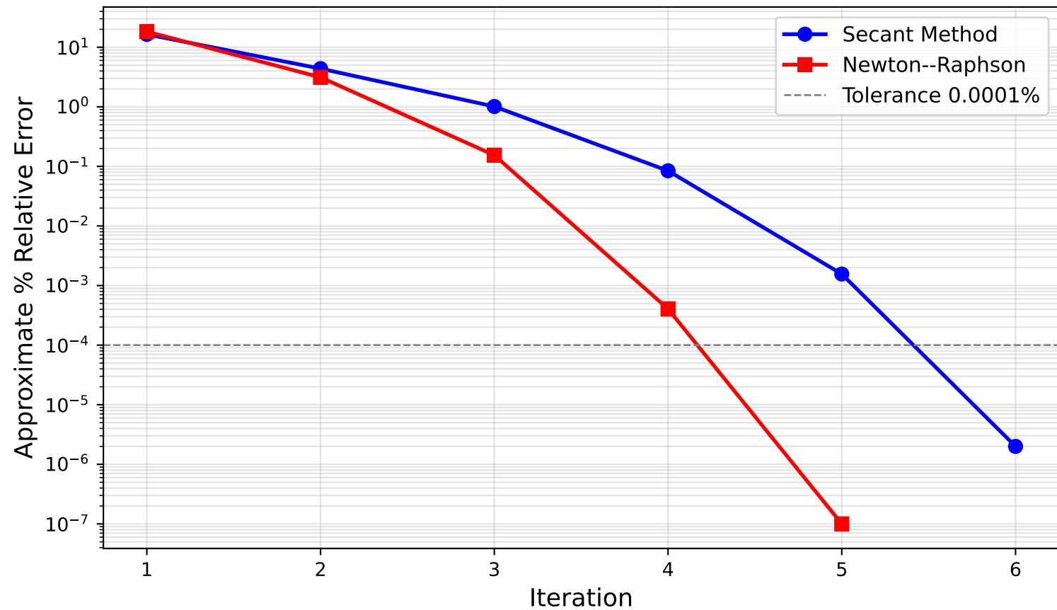
Error Convergence: Secant vs Newton--Raphson (Root 1, \theta_0 \approx 38^\circ )
