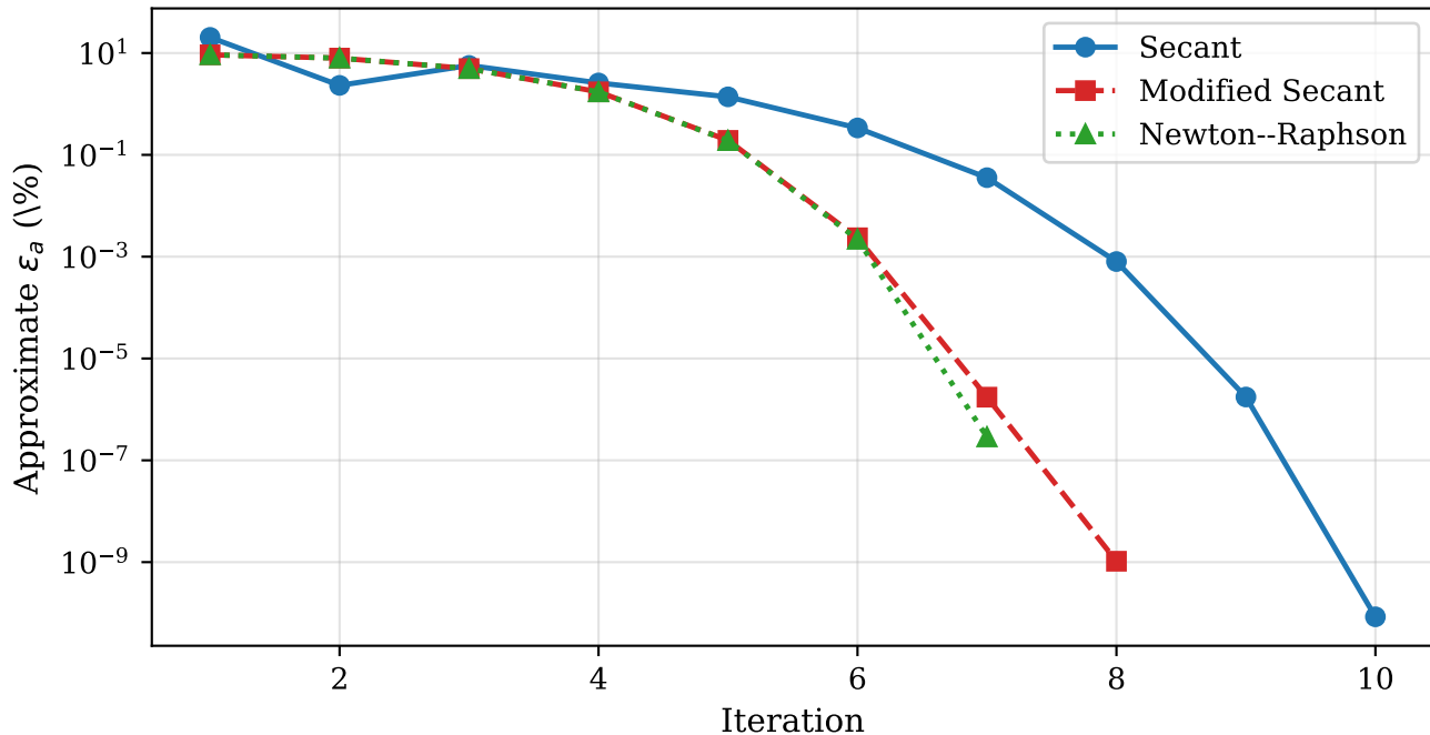
Error Convergence — Root 2 ( \theta^* \approx 51.53^\circ )
