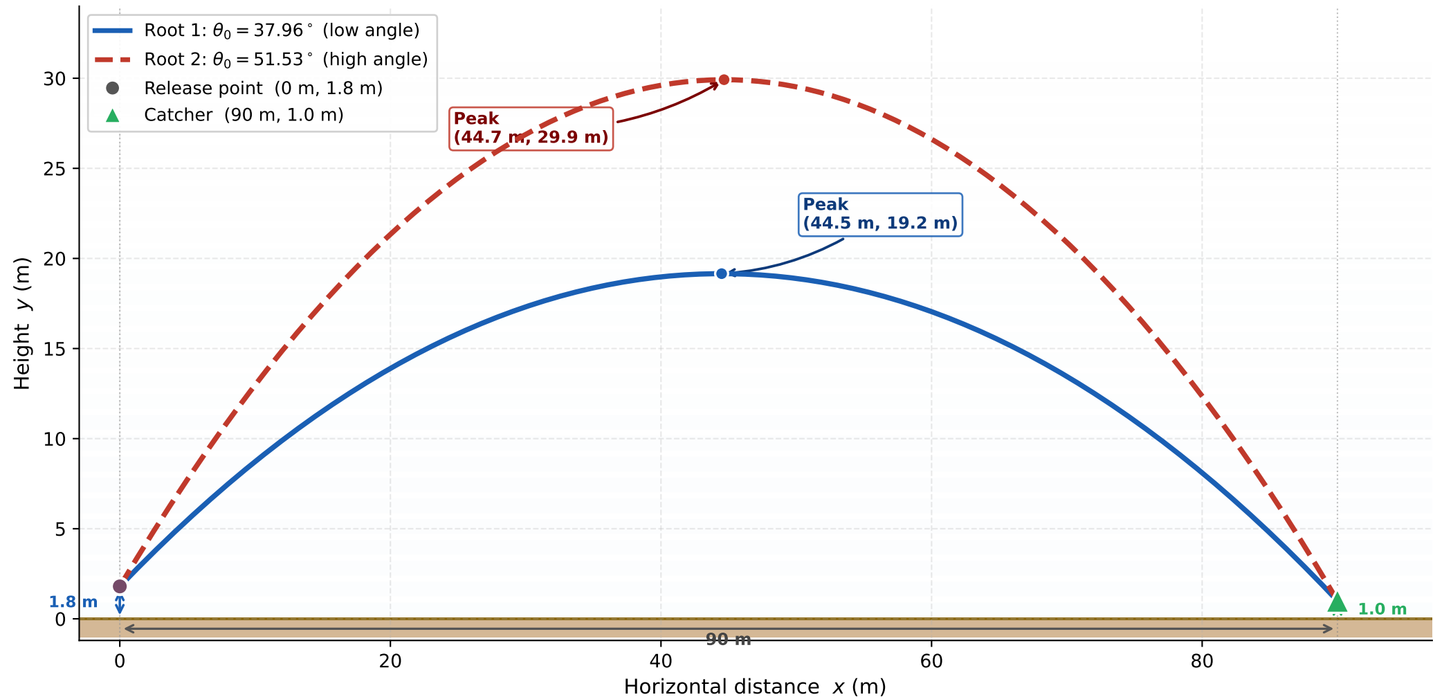
Ball Trajectories for Both Valid Launch Angles ( v_0 = 30 m/s, y_0 = 1.8 m, catcher at x = 90 m, y_c = 1.0 m)
