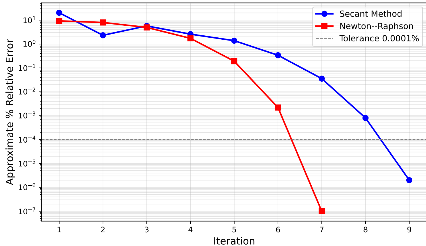
Error Convergence: Secant vs Newton--Raphson (Root 2, \theta_0 \approx 52^\circ )
